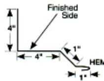
Side Wall 4x4x1x1x1/2
