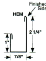
Jay 1/2x1x7/8x2 1/4x1/2
