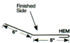
Break/Transition 6x8x1/2
