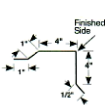
Gable 1x1x4x4x1/2 KO
