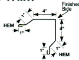
Corner - A/G 1/2x1x1x4x4x1x1/2
