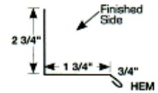
Starter Trim 2 3/4x1 3/4x3/4x1/2
