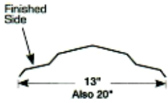
Ridge 13" & 20" wide
