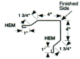
Corner - R 1/2x1x1 3/4x4x4x1 3/4x1x1/2
