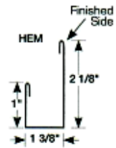
Head 1/2x1x3/8x2 1/8x1/2
