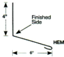
End Wall 4x6x1/2
