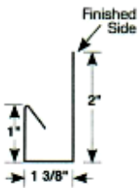
Jamb - R 1/2x1x1 3/8x2
